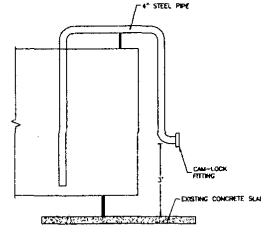
TYPICAL FILL/WITHDRAWAL PIPE SECTION N.T.S.
