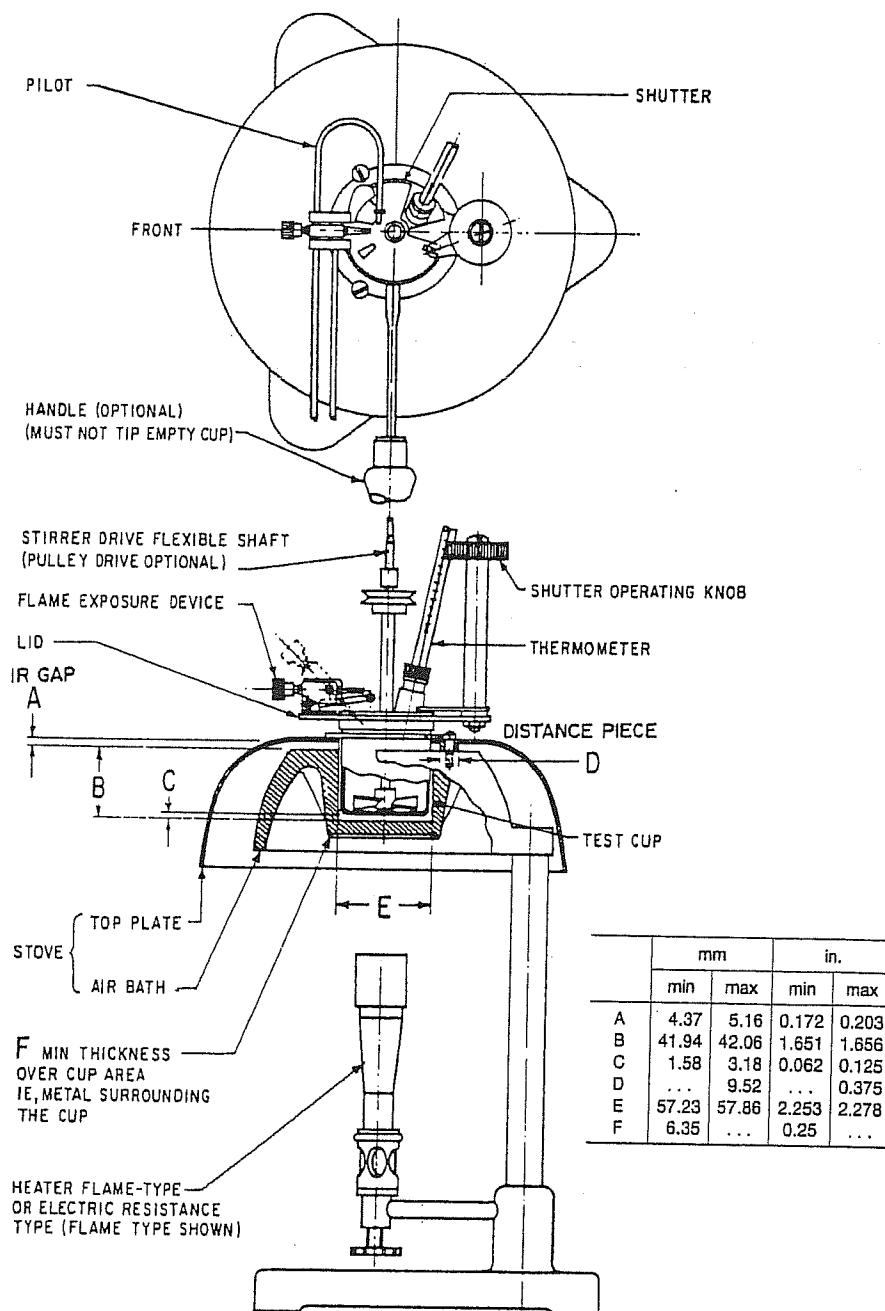
NOTE 1—Lid assembly can be positioned either right or left-handed. FIG. A1.1 Pensky-Martens Closed Flash Tester
