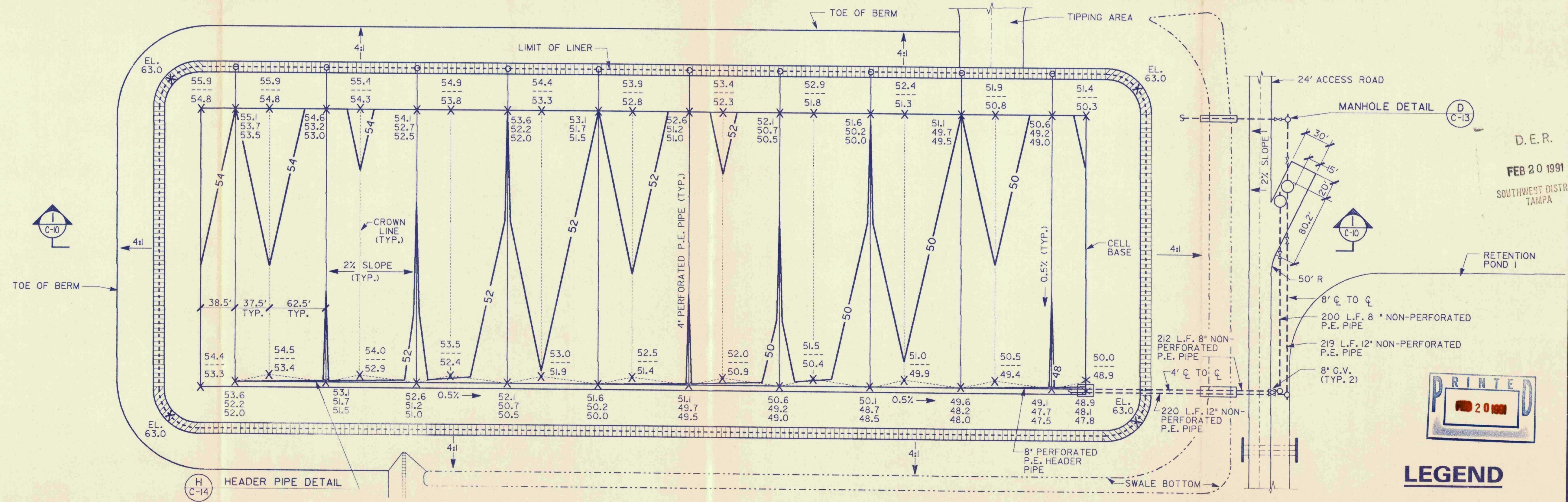
SECONDARY LEACHATE COLLECTION CELL A-1
