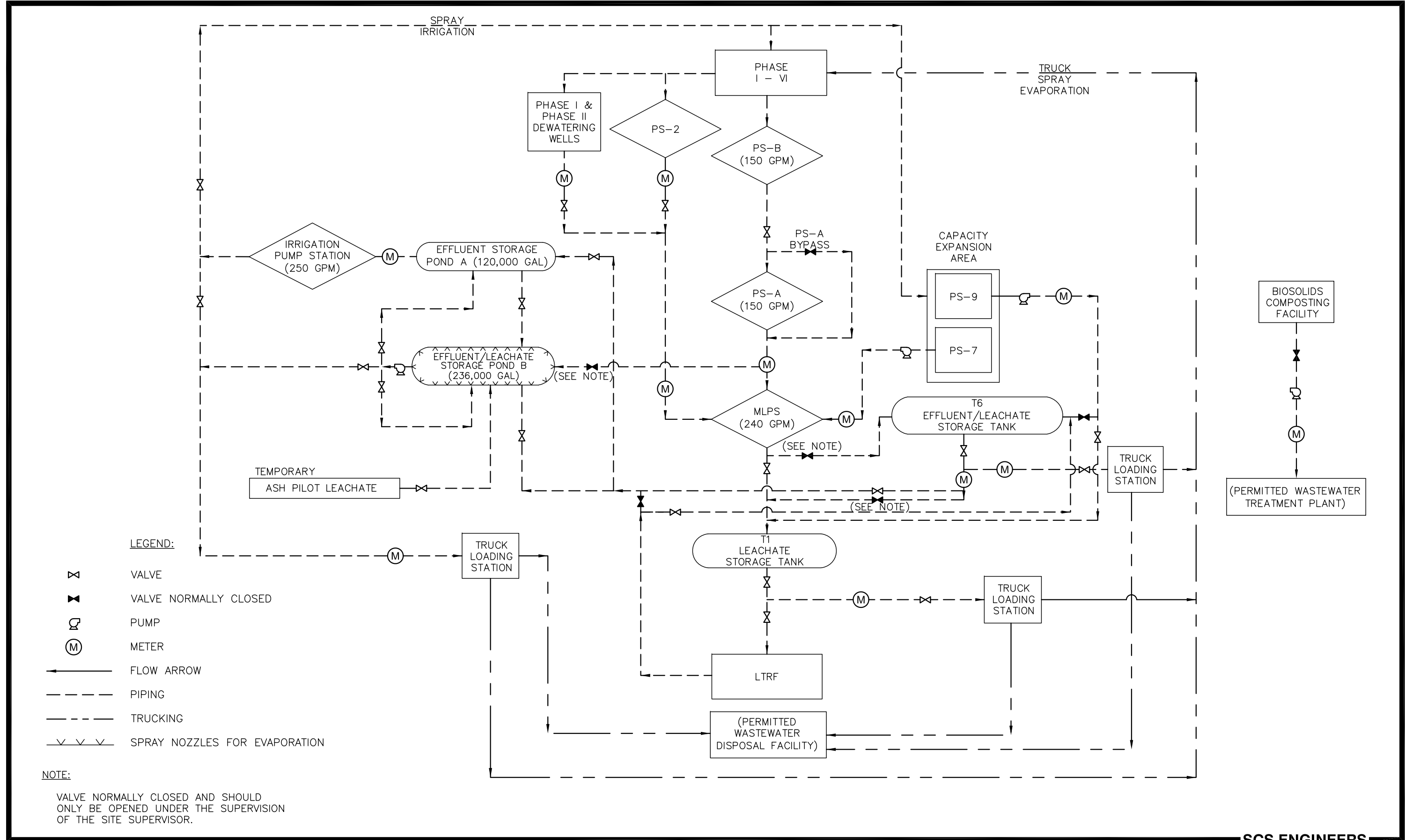
FIGURE 4-1. LEACHATE MANAGEMENT SYSTEM SCHEMATIC HILLSBOROUGH COUNTY JUNE 2020
