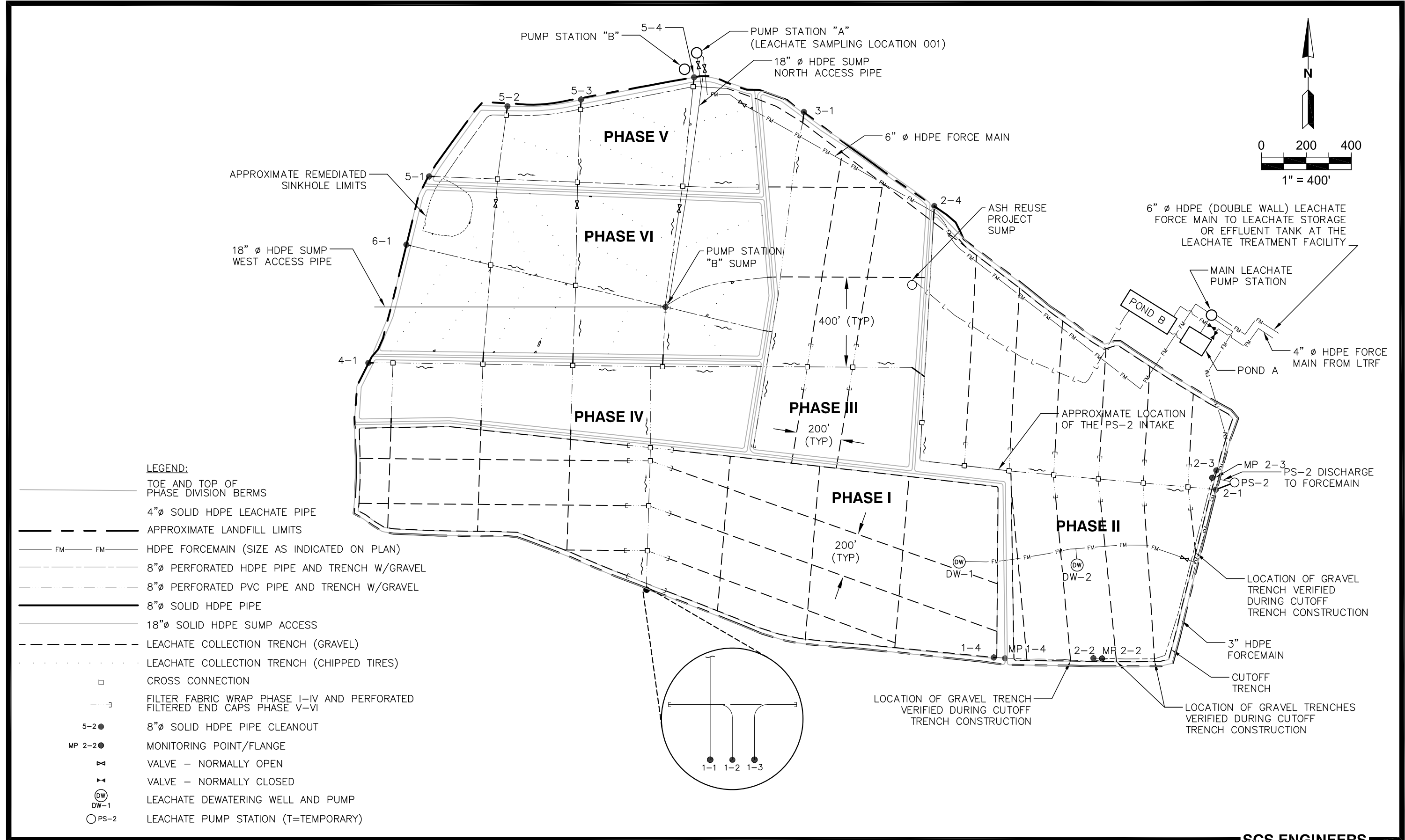
FIGURE 3-1. PHASES I-VI LEACHATE COLLECTION AND REMOVAL SYSTEM HILLSBOROUGH COUNTY JUNE 2020
