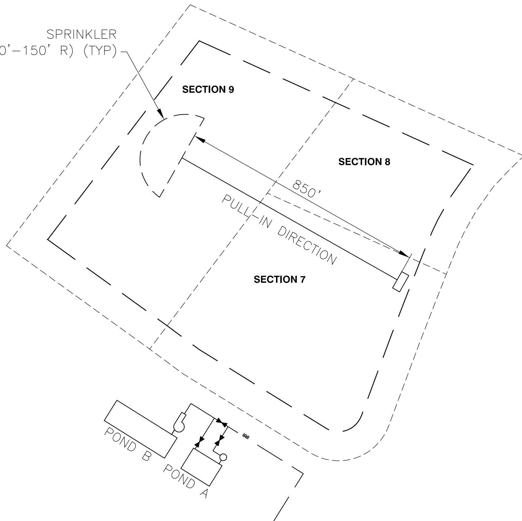
FIGURE 8-2. LOCATION OF CEA IRRIGATION SPRINKLER REEL HILLSBOROUGH COUNTY JUNE 2020
