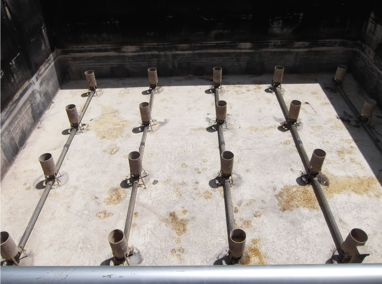
Photo 1: North Leachate Tank after the cleaning and removal of grit.
