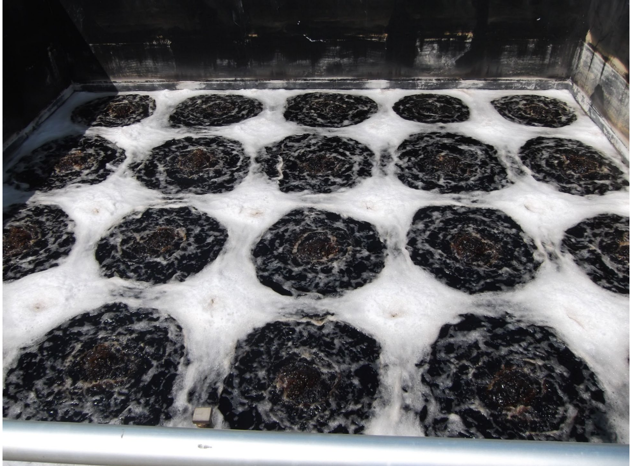
Photo 2: North Leachate Tank filled, and all diffusers are working as designed.
