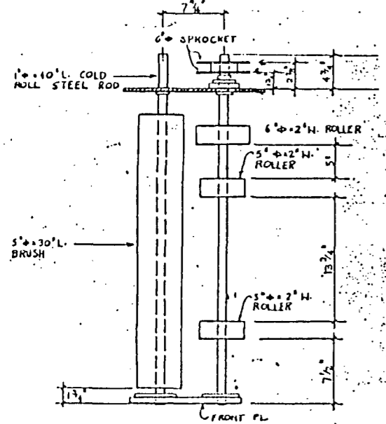
BTM. ASSEMBLY
