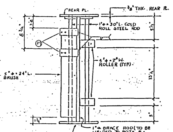
TOP ASSEMBLY
