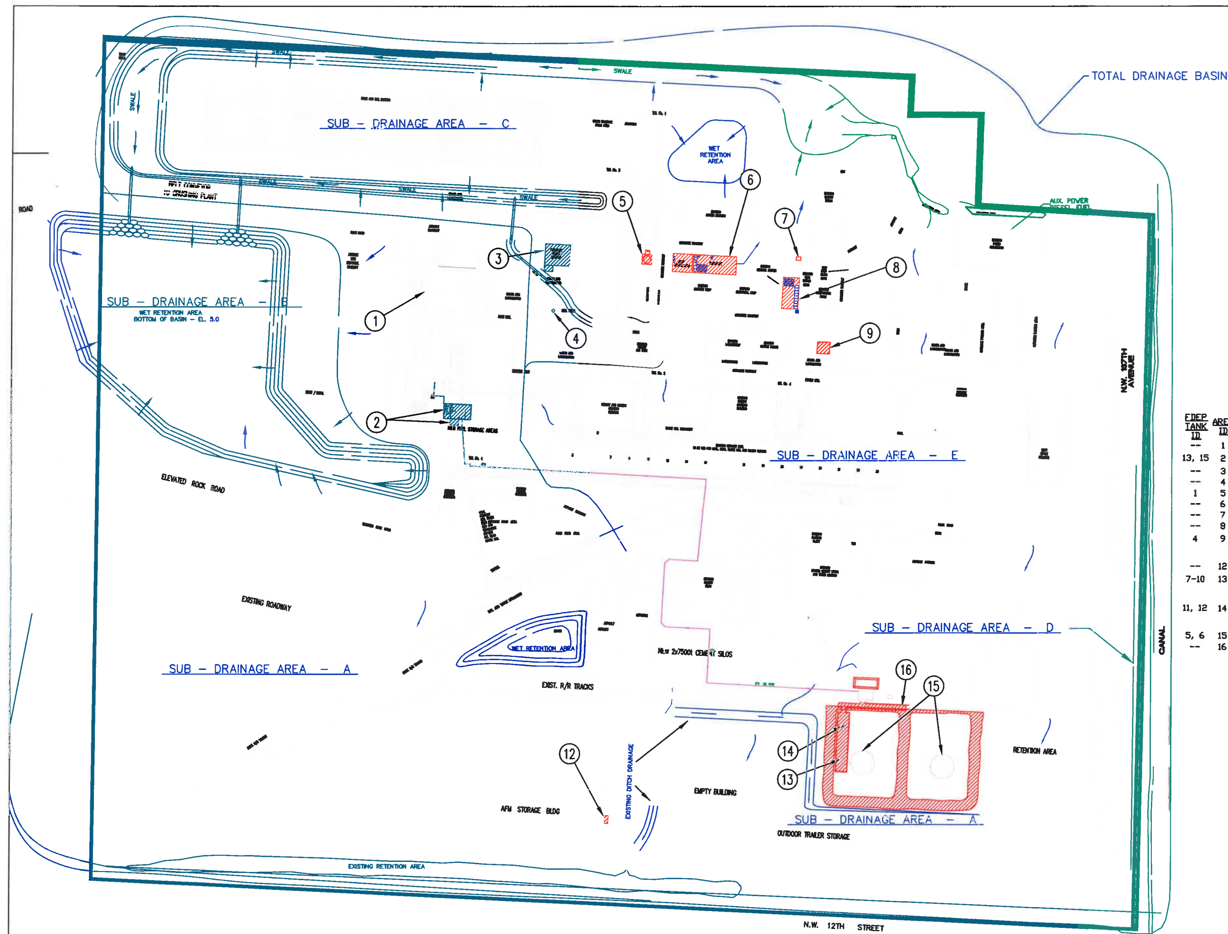
SPCC PLAN APPENDIX A, FIGURE 1- SITE PLAN CEMEX CONSTRUCTION MATERIALS FLORIDA, LLC MIAMI CEMENT PLANT MIAMI-DADE COUNTY, FLORIDA
