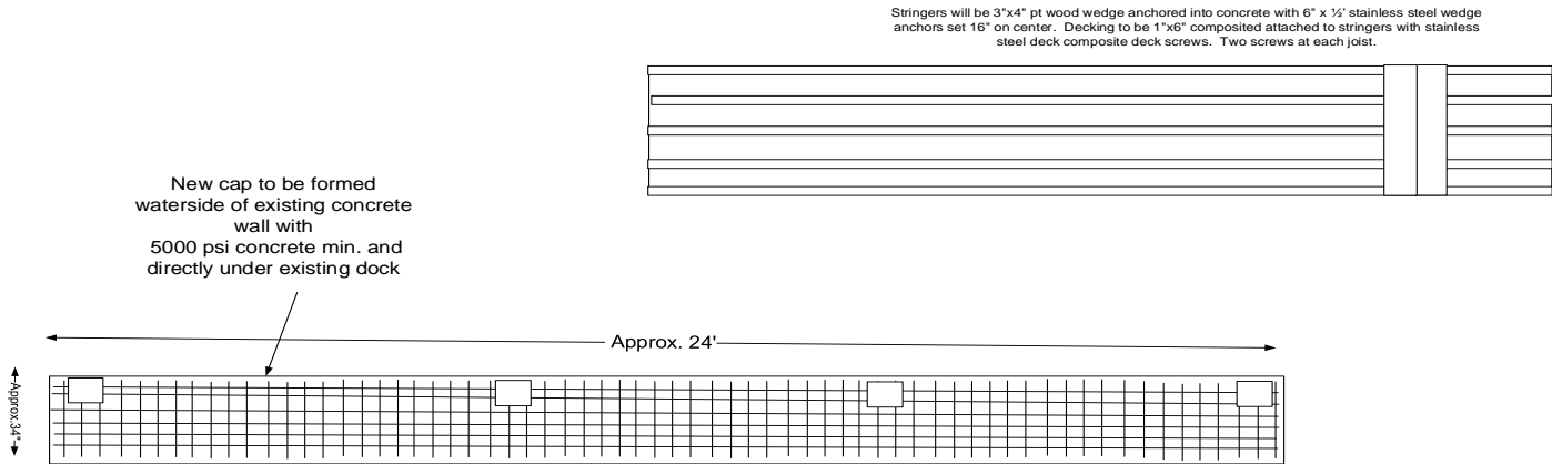
Top View new Concrete Cap
