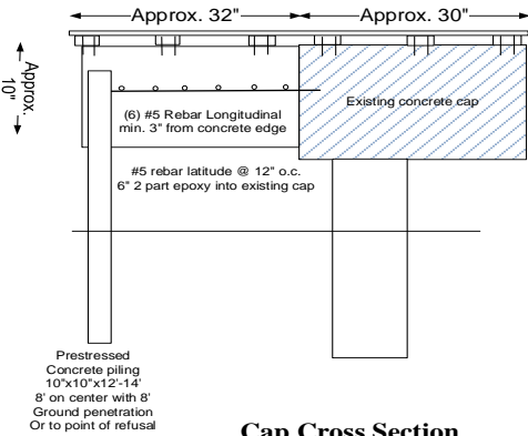
Cap Cross Section
