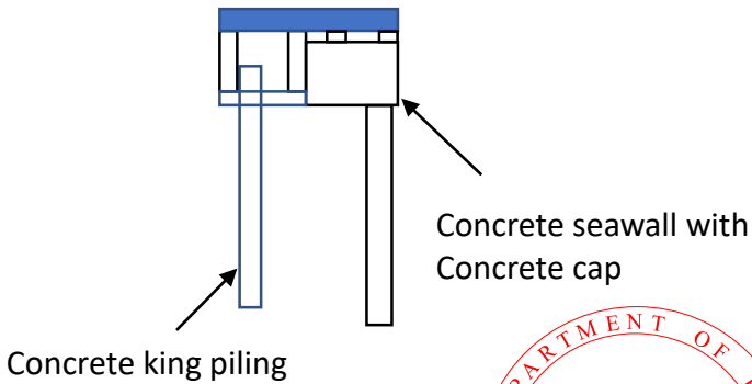
Dock Cross Section
