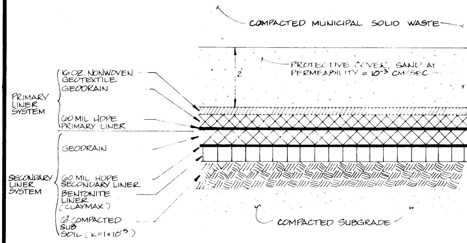
PRIMARY / SECONDARY LINER SYSTEM N.T.S.
