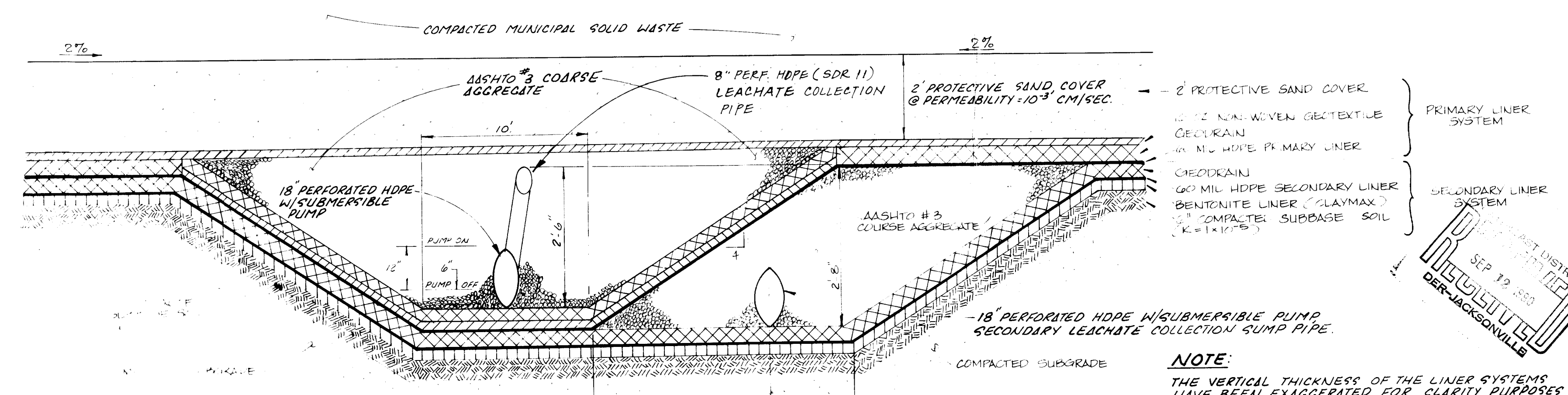
LEACHATE COLLECTION SYSTEM
