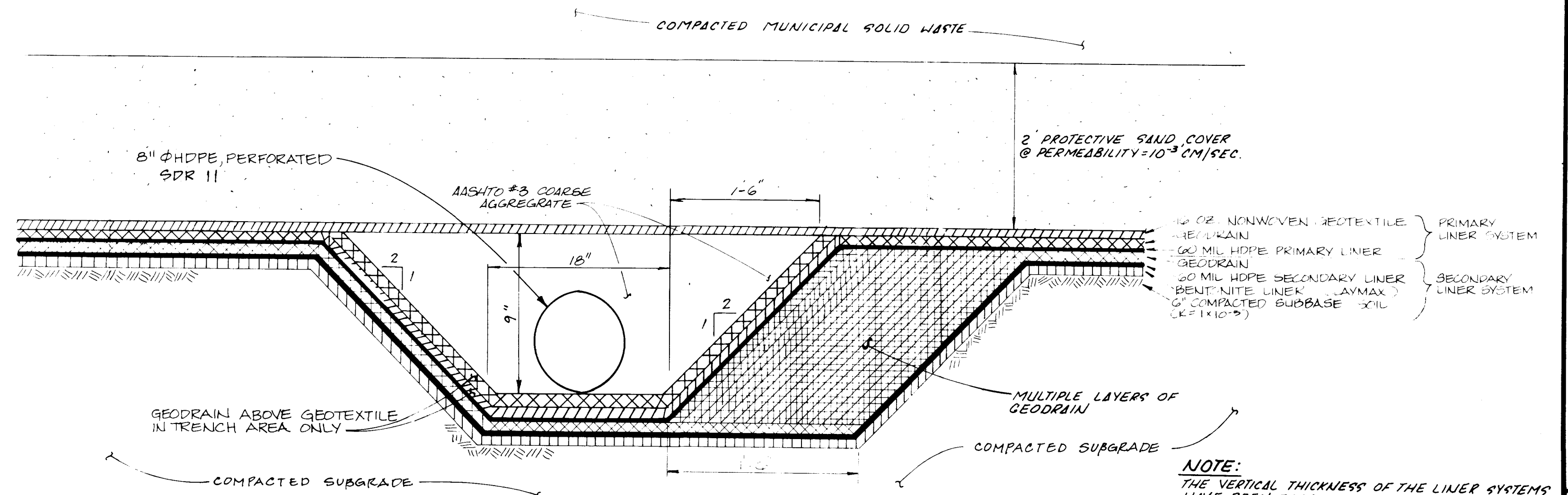
LEACHATE COLLECTION SYSTEM NTS
