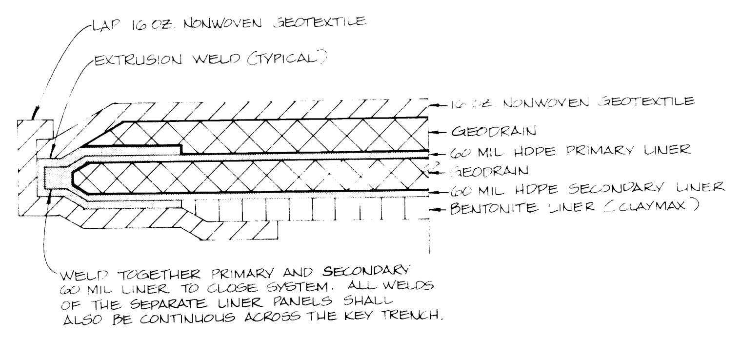
PRIMARY AND SECONDARY LINER END TREATMENT N.T.S.
