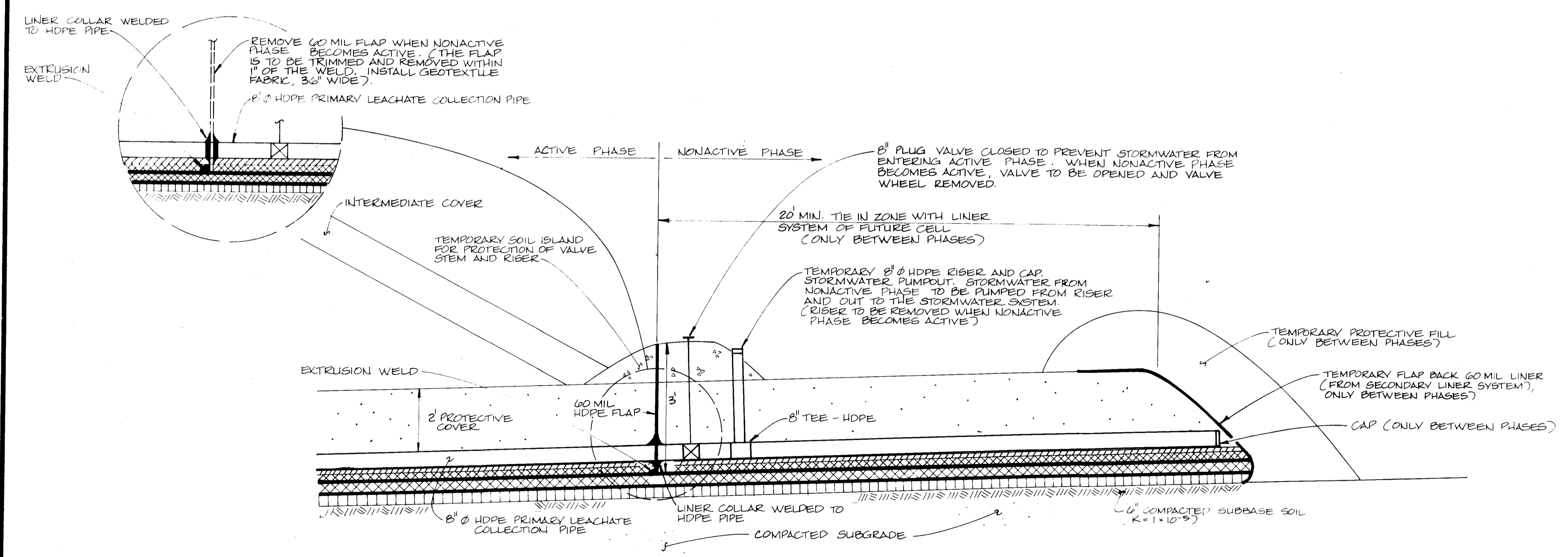
LEACHATE CONTROL FLAP BETWEEN NORTH-SOUTH PHASES N.T.S.
