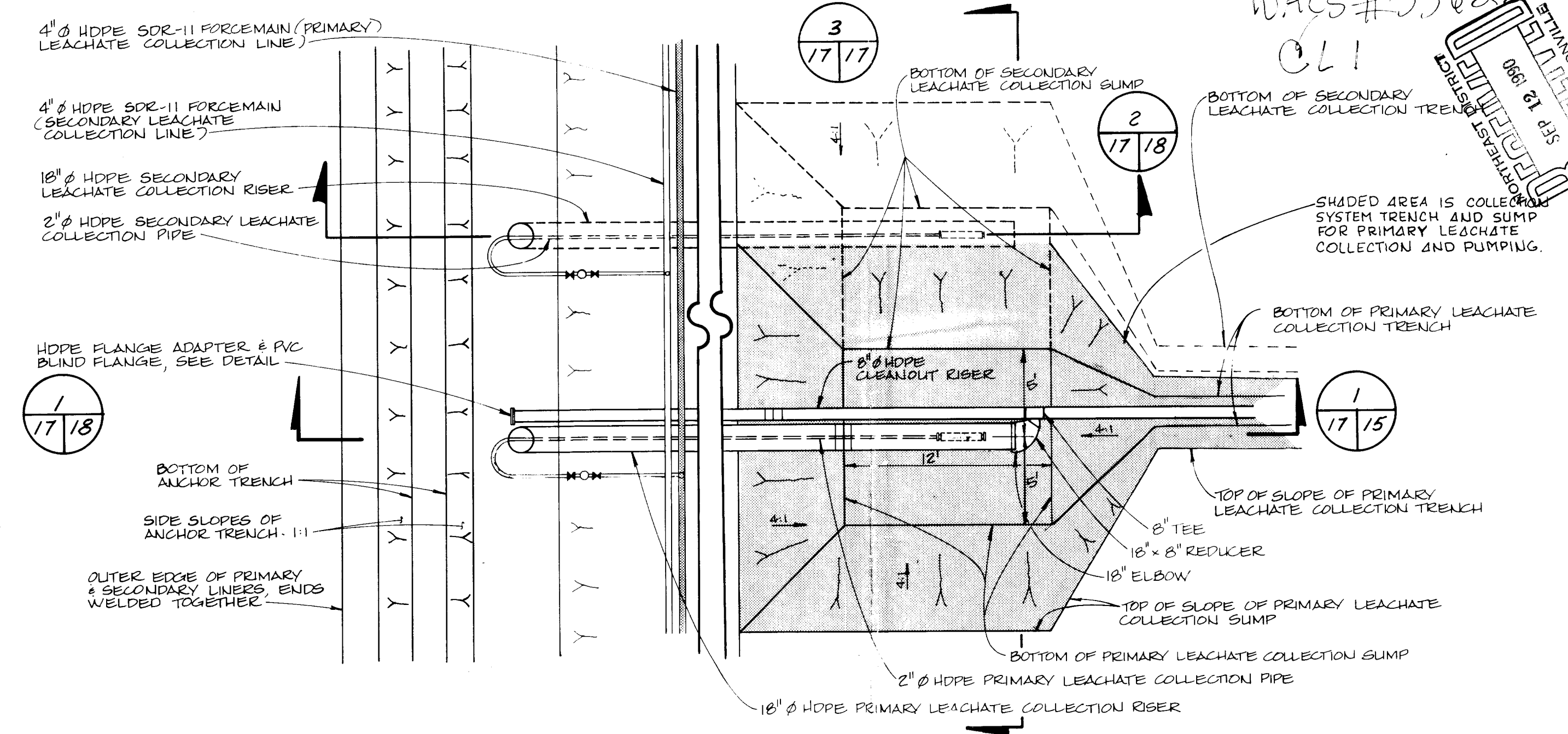
PRIMARY AND SECONDARY LEACHATE COLLECTION SYSTEM SUMP PLAN SCALE: 1" = 6'
