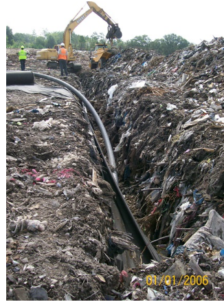
Horizontal Collector
