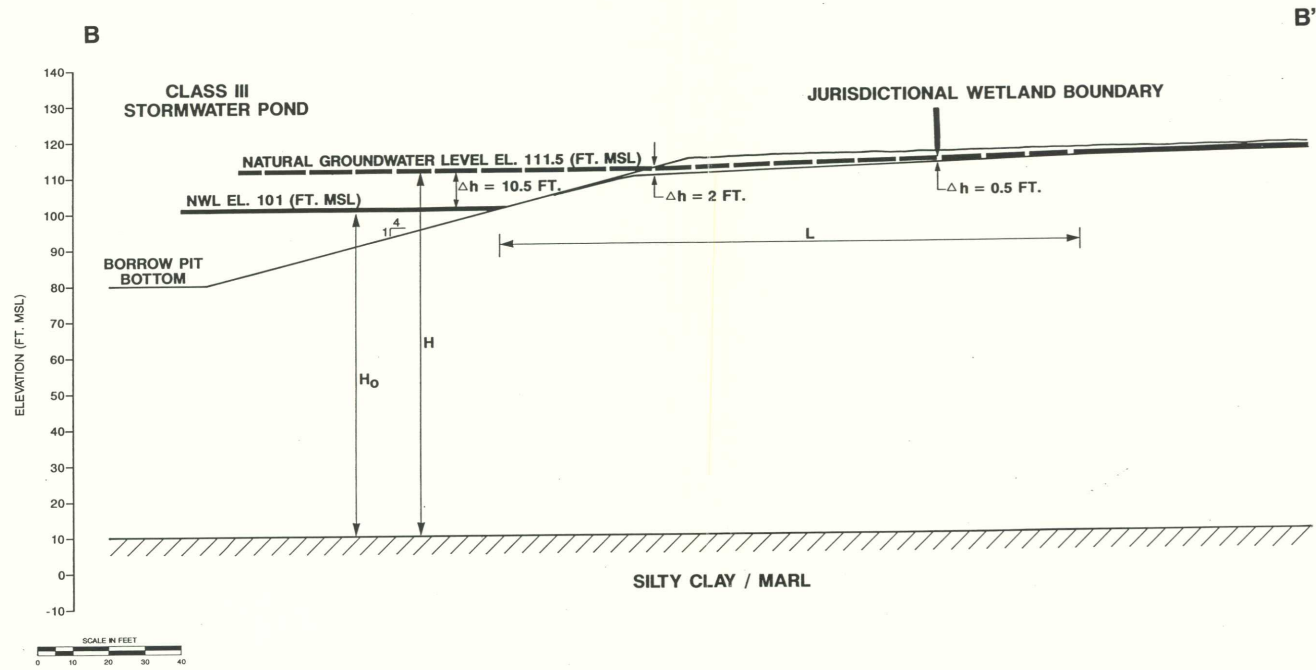
DRAWDOWN FROM CLASS III STORMWATER POND
