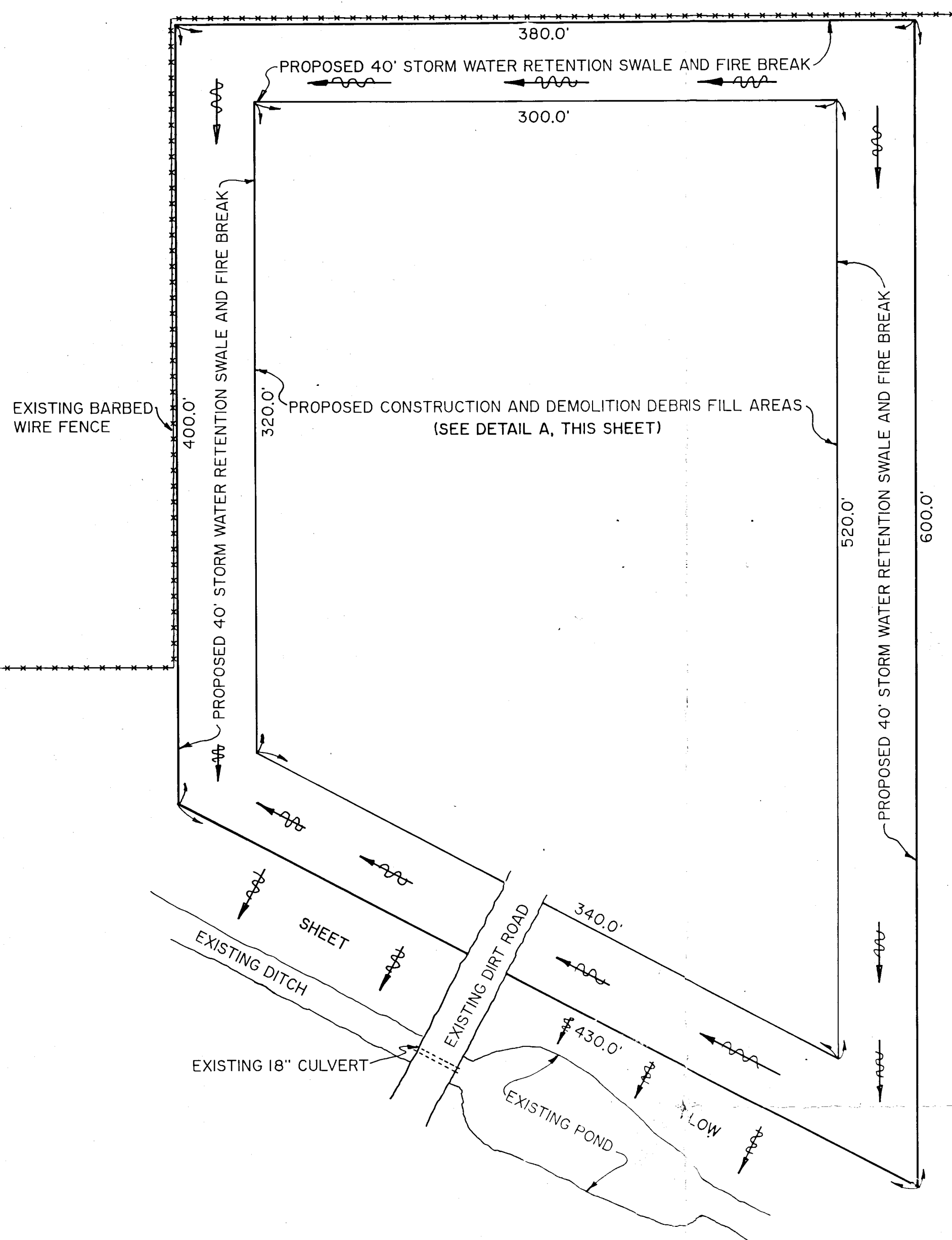
PLAN VIEW
