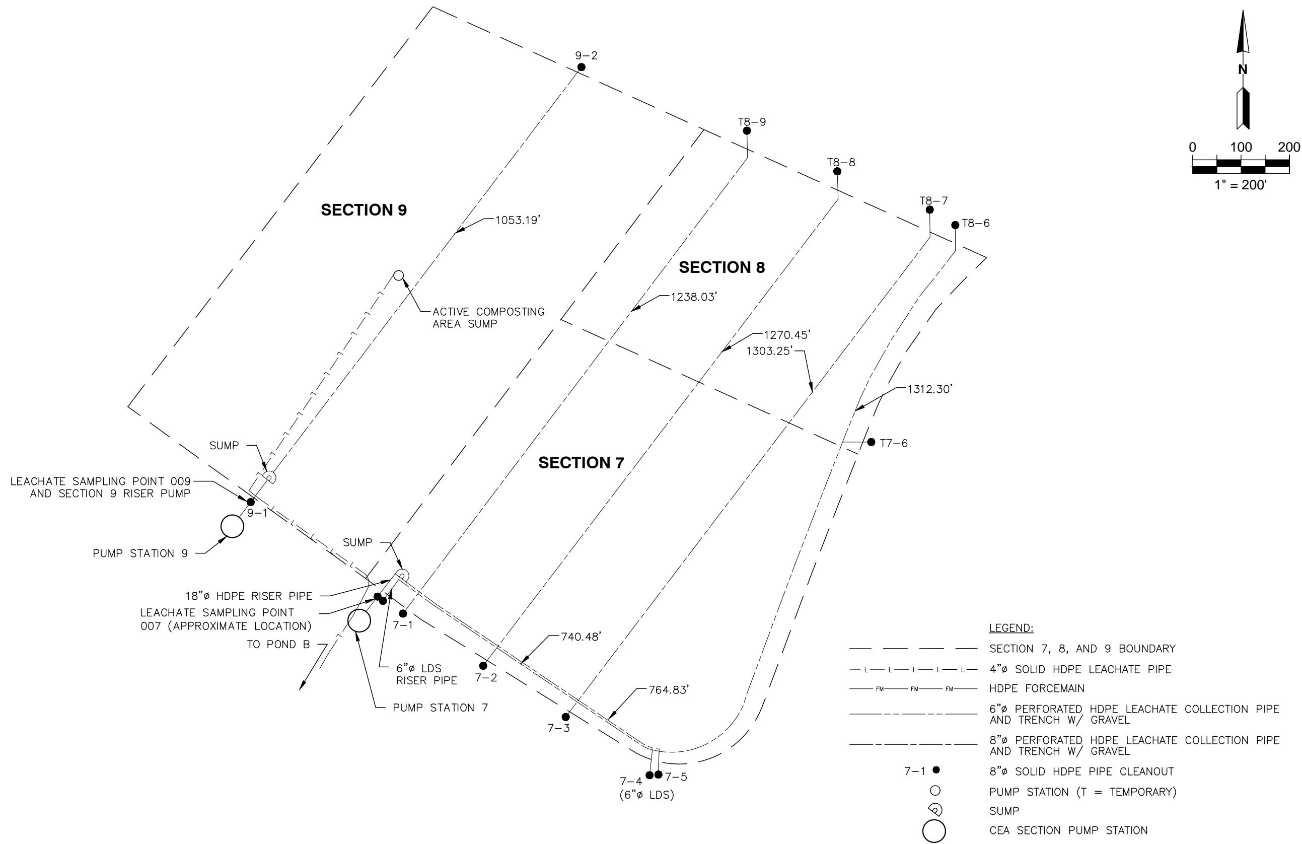
FIGURE 3.2. CAPACITY EXPANSION AREA (SECTIONS 7, 8, AND 9) - LEACHATE COLLECTION AND REMOVAL SYSTEM HILLSBOROUGH COUNTY OCTOBER 2018
