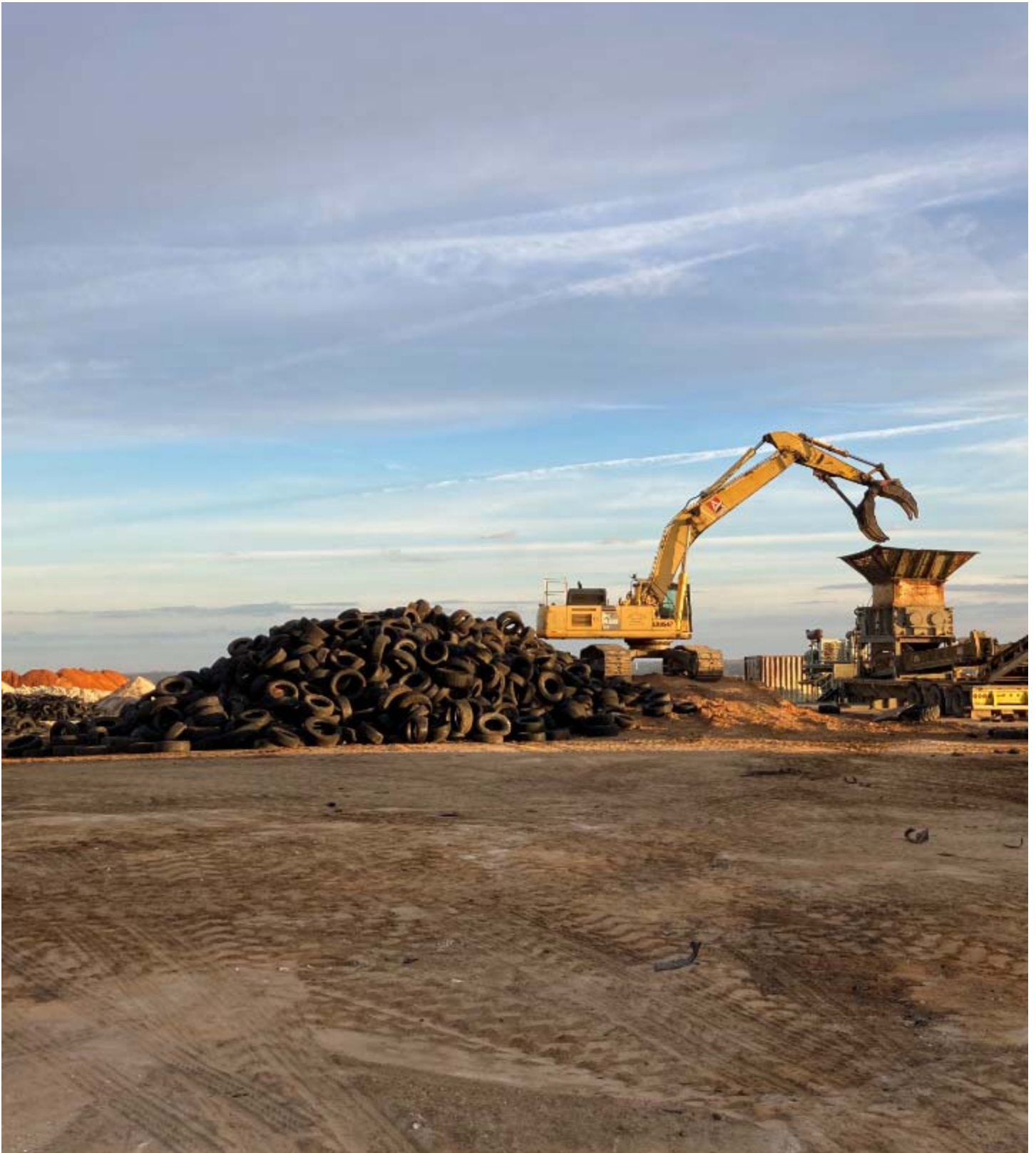
1 - Grapple feeding waste tires shredder
