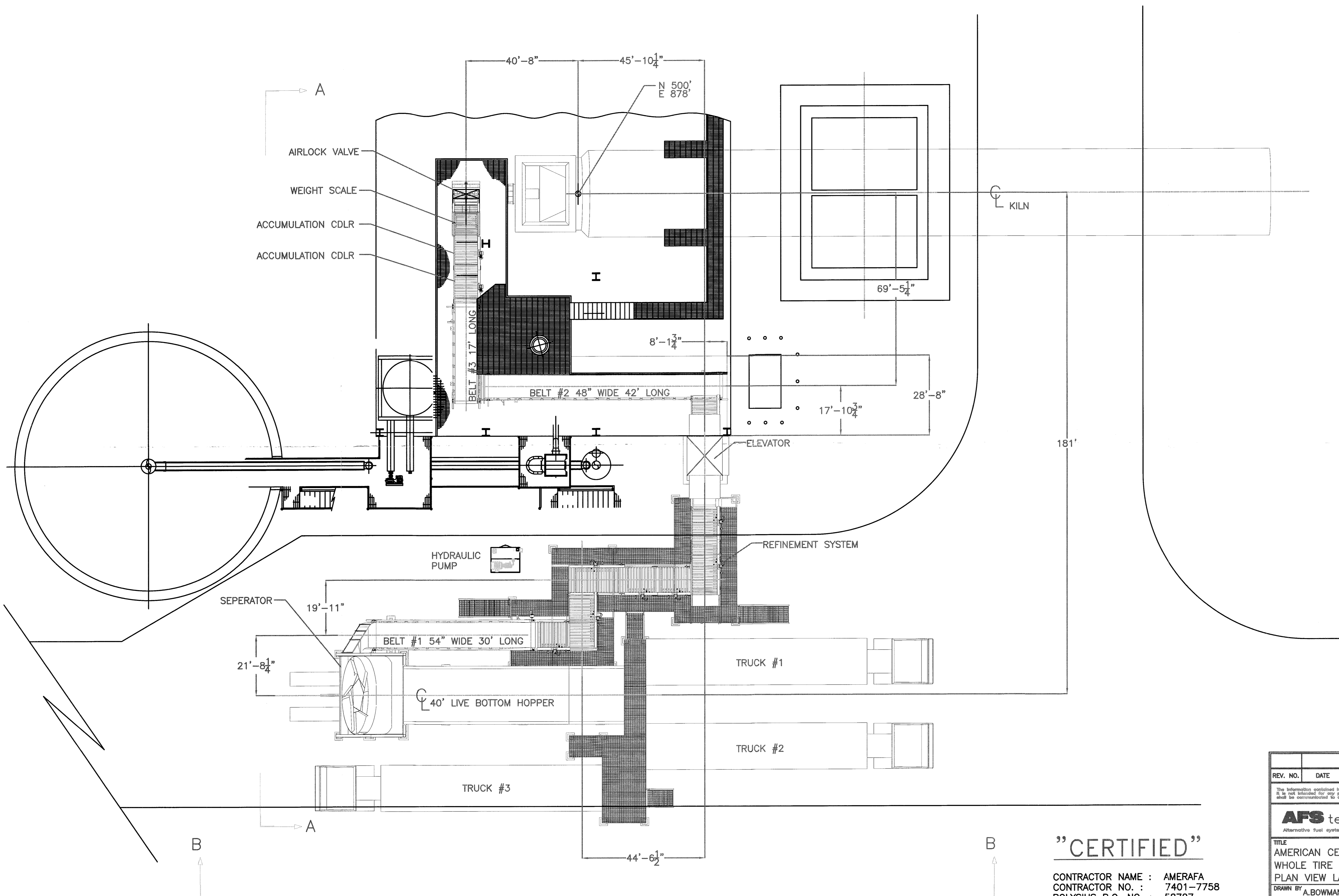
PLAN VIEW
