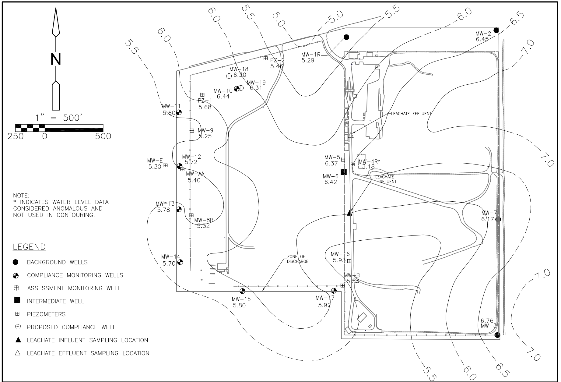
FIGURE NO. 1 GROUNDWATER CONTOUR MAP FLORIDAN AQUIFER CITRUS COUNTY CENTRAL LANDFILL WATER LEVEL DATA COLLECTED - JULY 20, 2009
